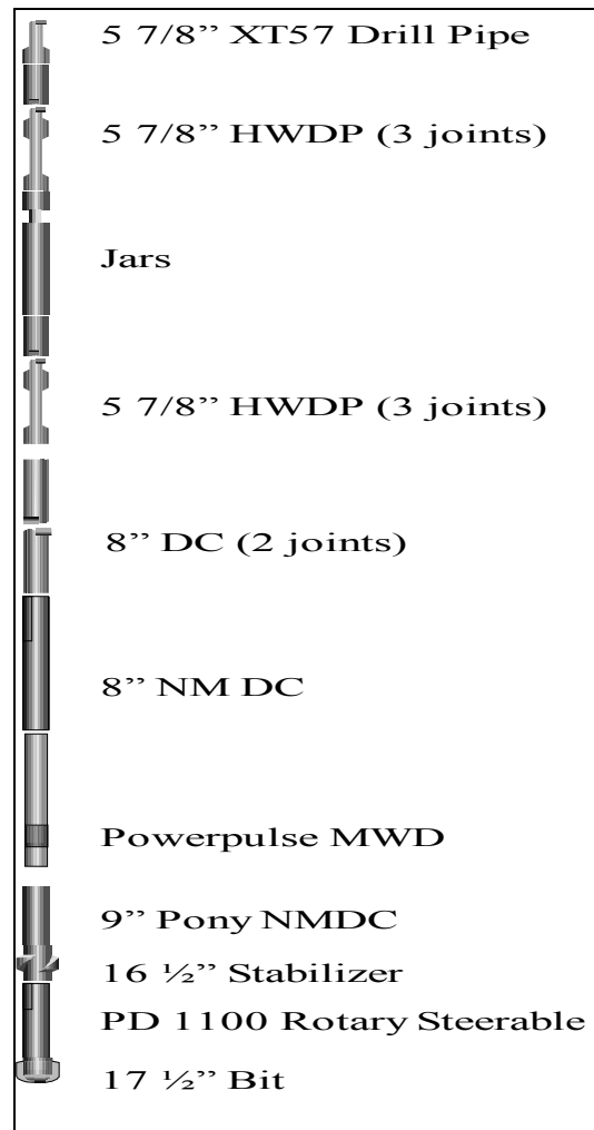
Figure 1 - Sample BHA - PD 1100 Tool + Xtra + 17 ½" BIT
