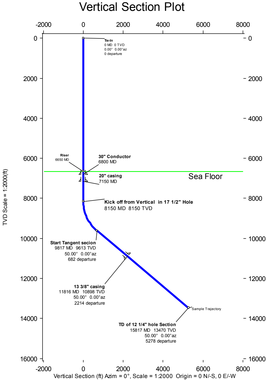
Figure 2 - Sample well trajectory – Vertical, Build and Hold in 17 1/2" Hole size
