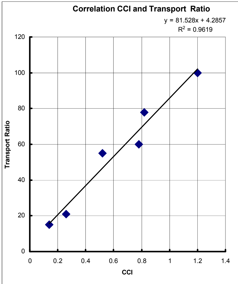
Figure 1 Correlation of Transport Ratio with CCI
