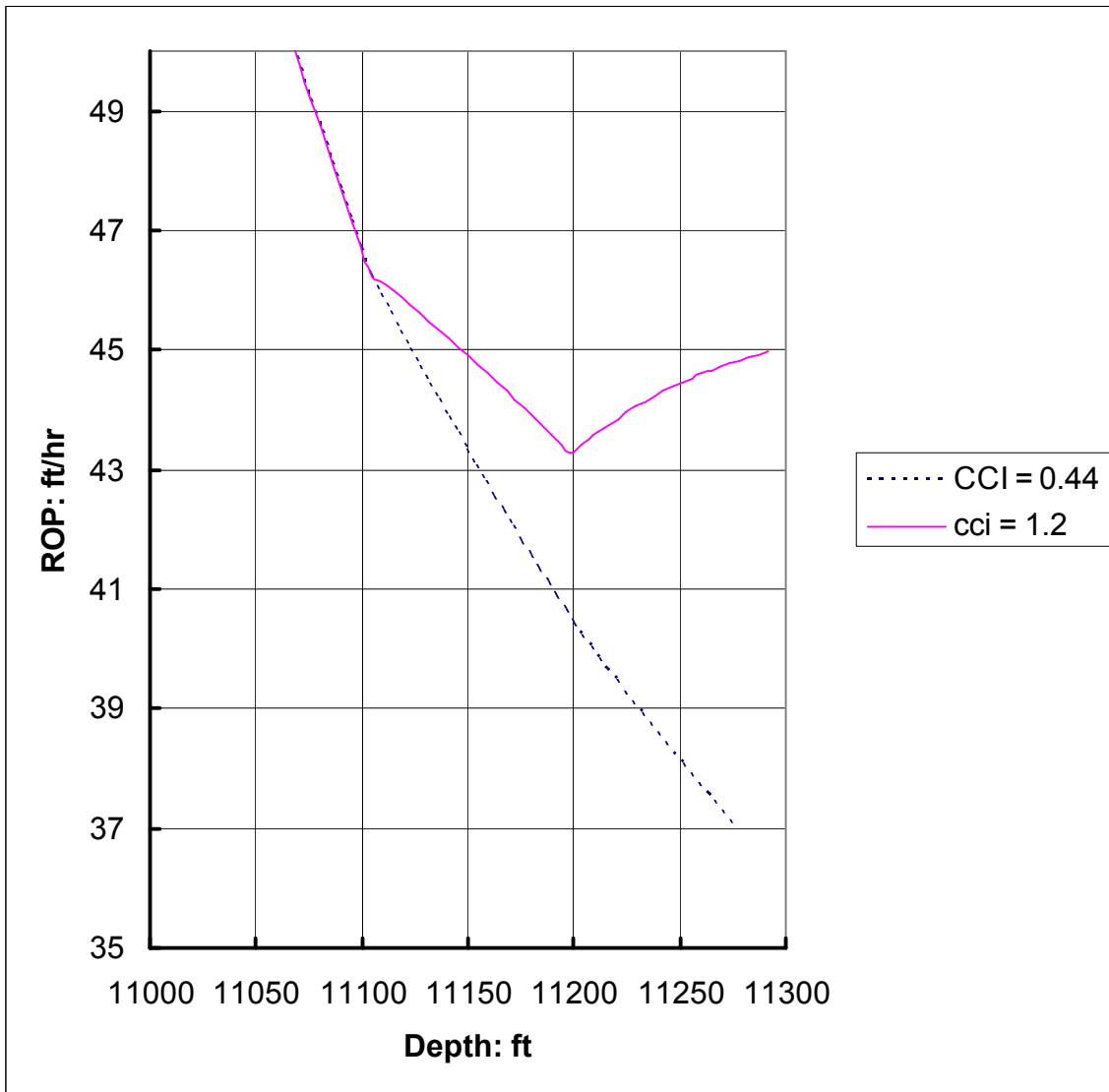
Figure 2 Effect of Carrying Capacity on Drilling Rate
