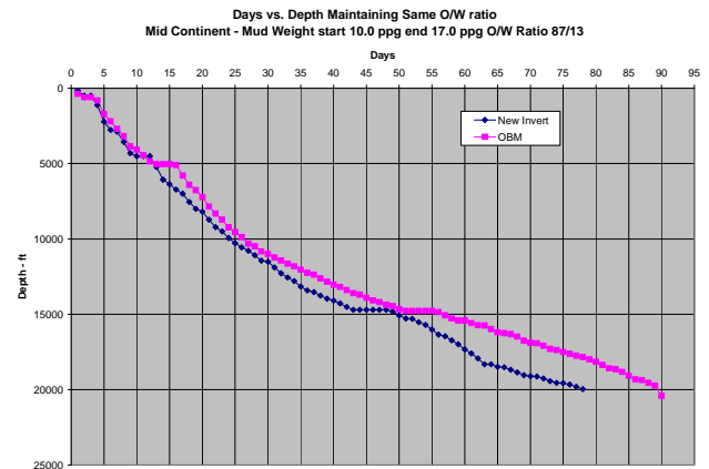
Fig. 1 – Comparison of drilling days vs depth.
