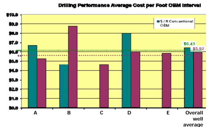
Fig. 2 – Comparison of drilling performance per interval by rig. (green is conventional invert, red is new one-drum system).
