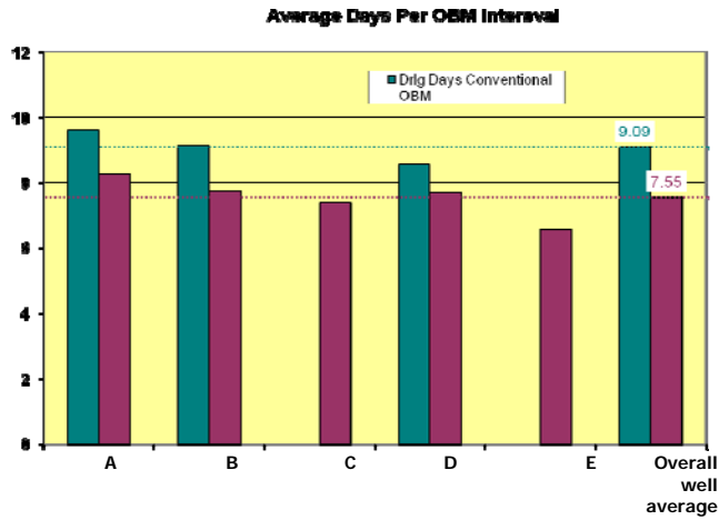
Fig. 3 – Comparison of average drilling days per interval by rig. (green is conventional invert, red is new one-drum system).
