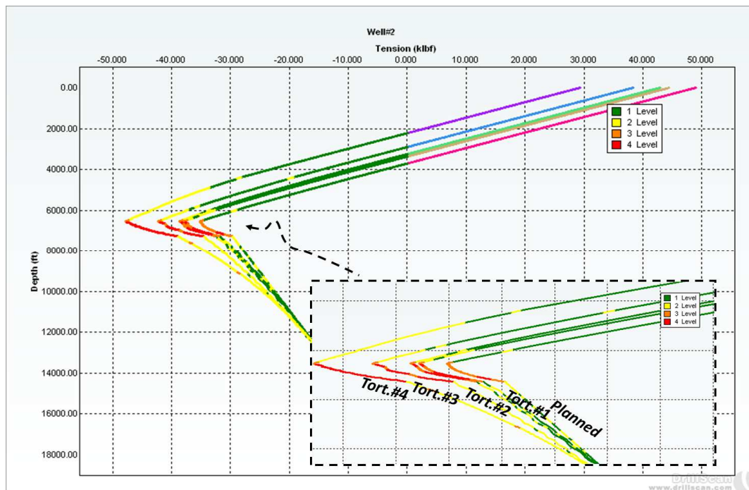
Figure 11: Tension/compression along the drillstring while running in hole @17,500ft - Buckling Severity Index – Wells #2 (Planned and different Tortuosity Levels)
