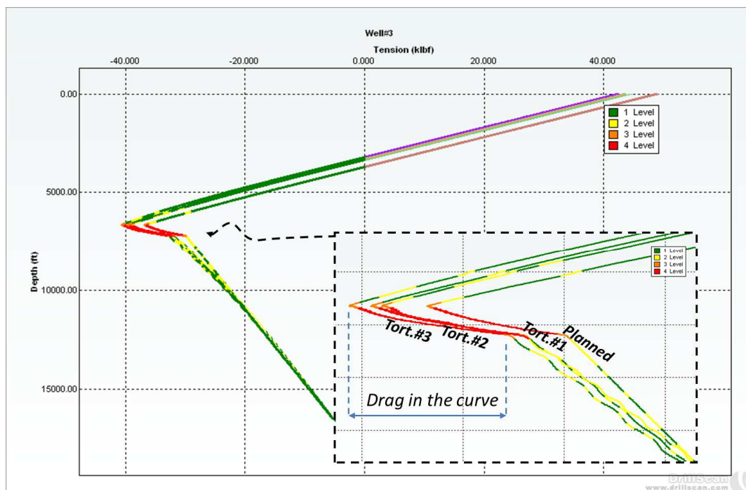
Figure 12: Tension/compression along the drillstring while running in hole @17,500ft - Buckling Severity Index – Wells #3 (Planned and different Tortuosity Levels)
