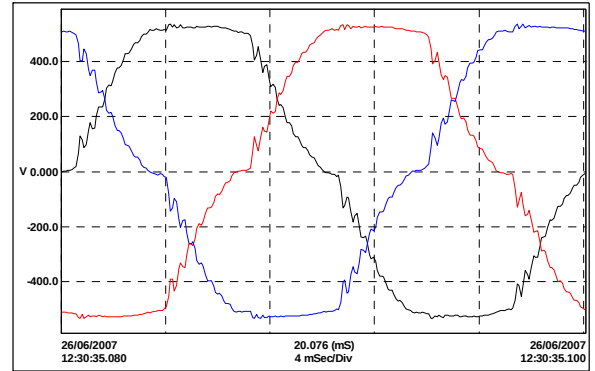
Fig 3 : Example of line voltages distorted by AC VFDs (8.8% Uthd) . Note - flat-topping at peak !
