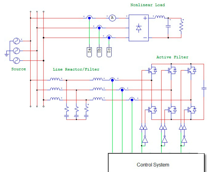
Fig 20: Parallel active filter schematic and connection
