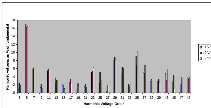
Fig 11 - Offshore oil platform harmonic voltage spectrum measured on 690V drilling package
