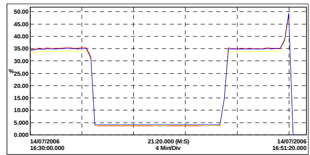
Fig 21 : Ithd on 3 x 900HP/630kW DC SCR drives without/with/without parallel broadband active filter. Ithd reduced from 35% to 3.7%
