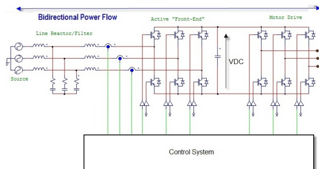
Figure 18 : Series active filter provides harmonic mitigation at input of an AC VFD (induction motor not shown)
