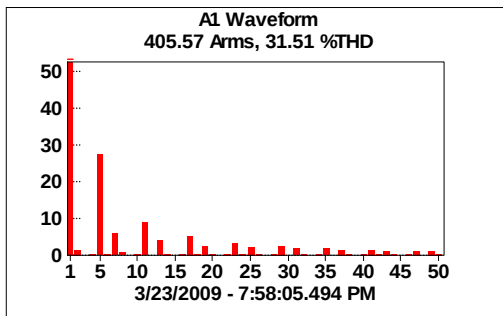
Fig 10 : DC SCR with line reactor. Typical harmonic current spectrum (%)
