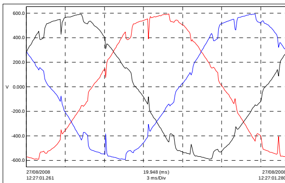
Fig 27 : 900HP DC drive line voltages with wide spectrum filter T type. Note - 1 x 700HP/500kW and 1 x 400HP/315kW untreated DC drives on same supply
