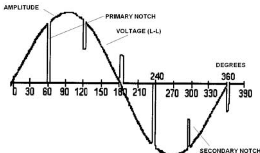
Fig 24 : Primary and secondary line notching
