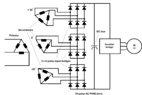
Fig 12 : Typical 18 pulse AC VFD with phase shift transformer
