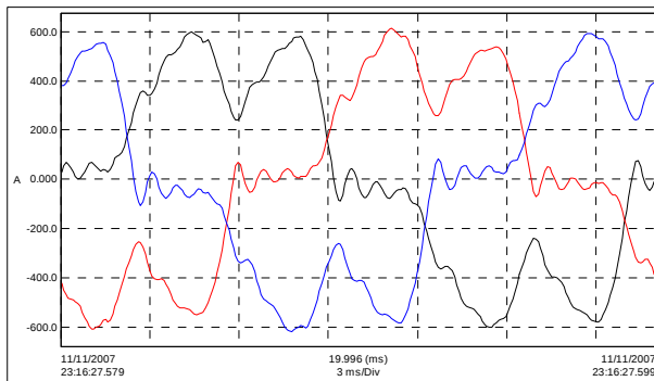
Fig 6 : Example of 1500HP (1100kW) VFD phase currents at moderate load. 34.88% I thd .
