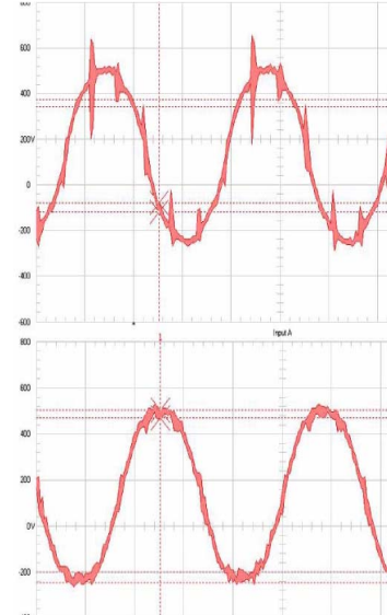
Fig 34 : The input (upper trace) and output (lower trace) to/from a wide spectrum filter on a DC drilling package. The sensitive VFDs are connected to the lower trace.
