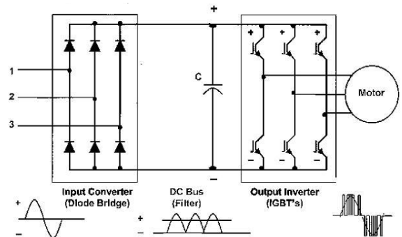
Fig 4 : Simplified 6 pulse AC VFD schematic
