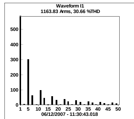
Fig 16 – 900HP/630kW DC SCR drive harmonic current spectrum. No mitigation – 30.66% I_{thd}
