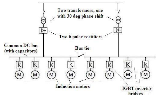
Fig 8 : Common DC bus system with quasi 12 pulse harmonic mitigation configuration
