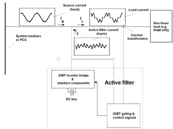
Fig 19 : Parallel active filter current waveforms
