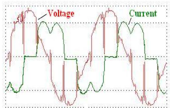
Fig 26 : Severe line notching on due to fully controlled SCR rectifiers on DC drilling package
