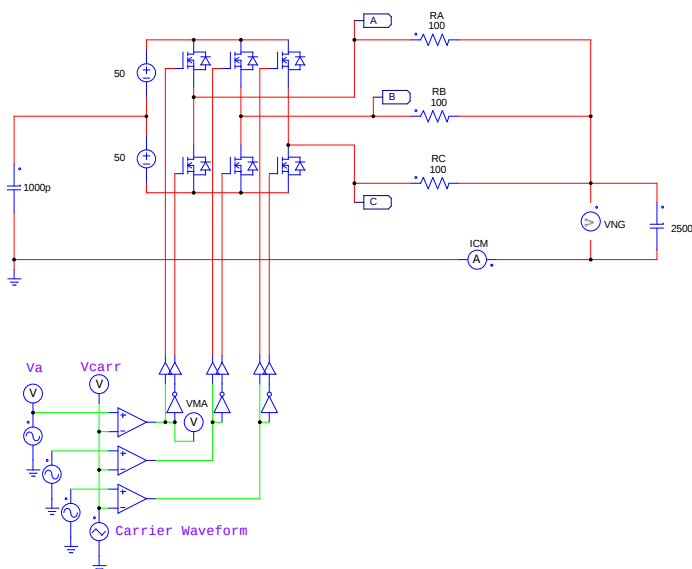
Figure 36 : Simplified circuit for common mode shift
