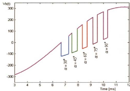
Fig 32 : Notch depth variations on firing angle changes
