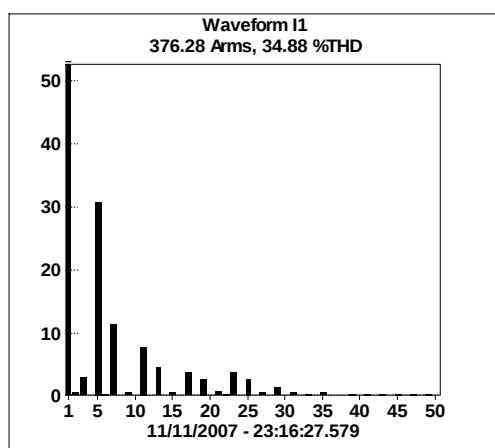
Fig 7 : Example of 1500HP (1100kW) VFD current harmonic spectrum (%). (Fundamental rescaled to 50% to show detail. Partial resonance at 23 rd and 25 th harmonic)
