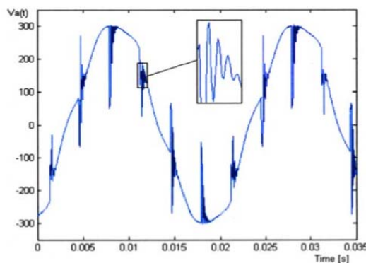
Fig 33 : Example of line notches and voltage oscillations due to delay angle of 45 deg
