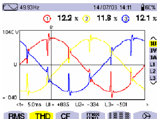
Fig 28 : 3 x 900HP DC drives voltage waveforms with 3% AC line reactors only
