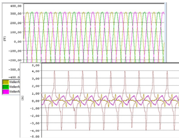
Fig 45 : Examples of live voltage and current waveforms. These can be expanded into single cycle waveforms
