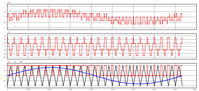
Figure 37 : Top: Motor Drive Line to neutral voltage Middle: Neutral to ground voltage Bottom: IGBT modulation on phase A, all waveforms are shown without parasitic capacitance connected
