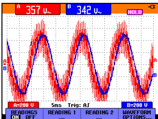
Fig 40 : Red trace represents Phase V1 to ground voltage when the draw-works and/or top drive is assigned or running
