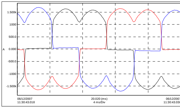
Fig 9 – Example of DC SCR drive at moderate load (31.51% Ithd)
