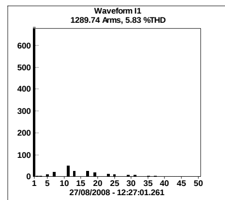
Fig 17 – 900HP/630kW DC SCR drive harmonic current spectrum (I1) in AMPS. With T type wide spectrum filter - 5.83% I_{thd}
