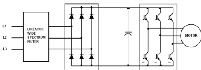
Fig 14 : Advanced wide spectrum filter connection to VFD. Can also be connected to a group of AC or DC drives.
