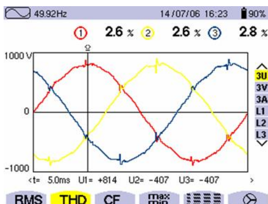
Fig 29 : 3 x 900HP DC drives voltage waveforms with active harmonic filter and 3% AC line reactors.
