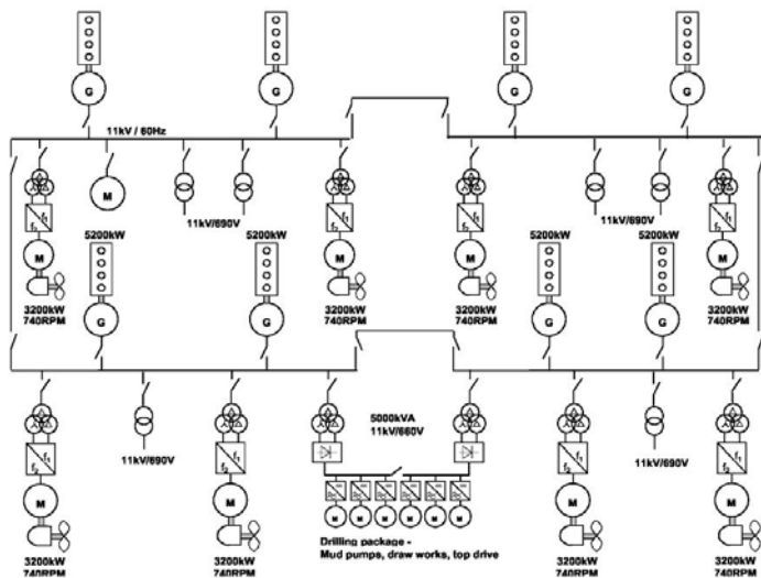
Fig 2 : Typical DP3 semi-submersible drilling rig
