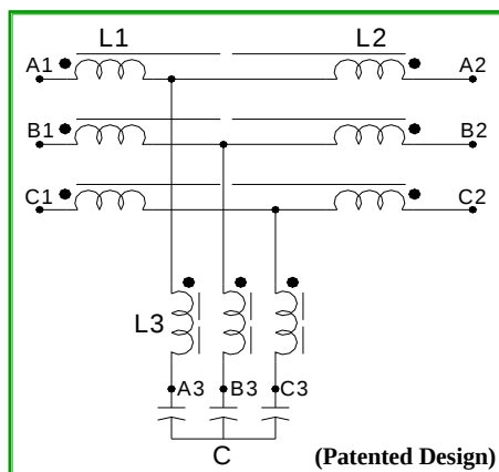
Fig 13 – Advanced wide spectrum filter schematic.
