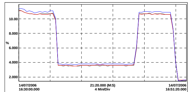
Fig 22 : Uthd on 3 x 900HP/600kW DC drives without/with/without parallel broadband active harmonic filter. Uthd reduced from 11.2% to 3.2%.
