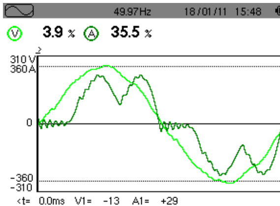
Fig 5 : One phase of VFD input (voltage and current) waveforms
