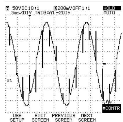
Fig 30 : Voltage spikes due to large DC SCR drives
