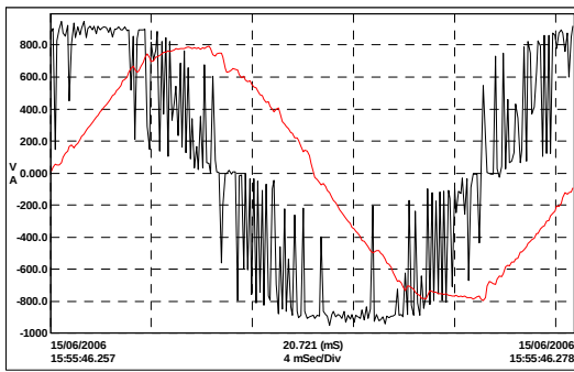
Fig 35 : Typical VFD output voltage (black) and current (red) waveforms.
