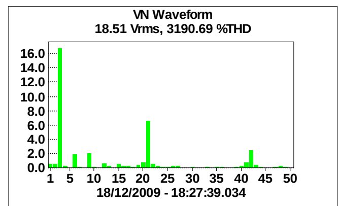
Fig 42 : Phase 1 to ground voltages on EMC compliant VFD drilling package. Note - two VFDs systems running.
