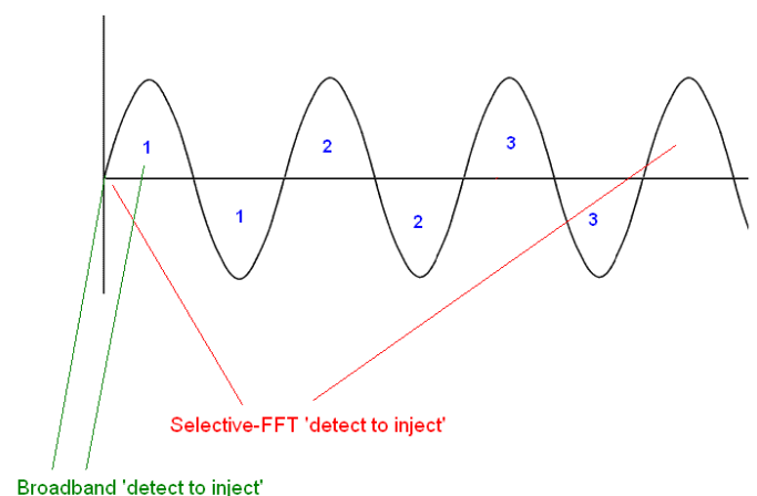
Fig 23 : Comparison of 'broadband' and 'selective FFT' active filter response times
