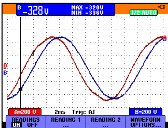
Fig 39 : Red trace represents typical Phase V1 to ground voltage when neither the draw-works and/or top drive VFDs are assigned or running
