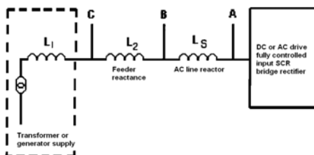
Fig 25 : Line impedance distribution and the effect of line notching
