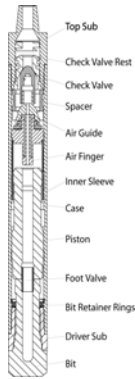
Figure 1 -- Air Hammer
