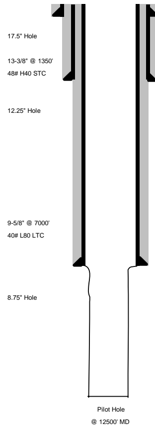
Figure 7 -- Well Bore Schematic
