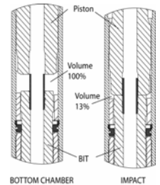
Figure 6 -- Conventional Air Hammer Bottom Chamber Compression (87%)
