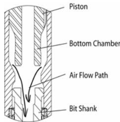
Fig 4 Deep-Hole Oilfield Air Hammer (No Foot Valve)
