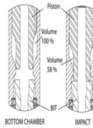
Figure 5 -- Oilfield Air Hammer Bottom Chamber Compression (42%)
