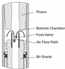
Fig. 3 Conventional Air Hammer (Foot Valve can break)
