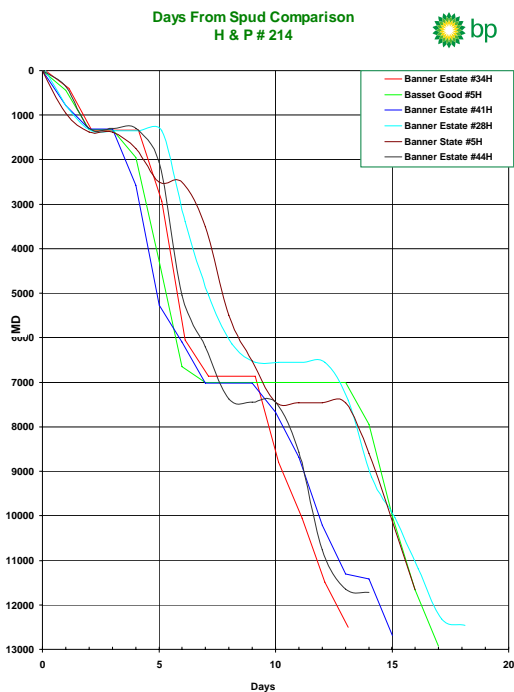
Figure 8 -- Days VS Depth Curves
