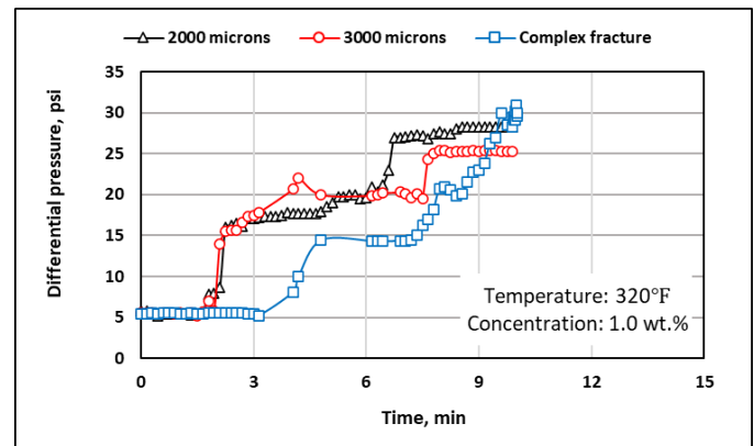
Figure 7 – Sealing performance of shape memory polymer at different fracture sizes
