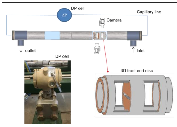
Figure 3 – Modified schematic design of the main test section.
